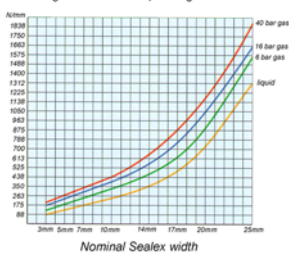
Average surface stress per length of Sealex
