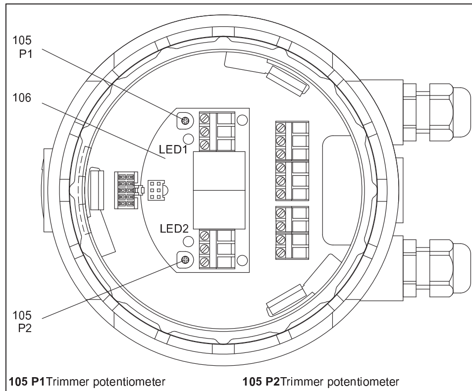
Diagram 19 Way-switch printed circuit board in cover
