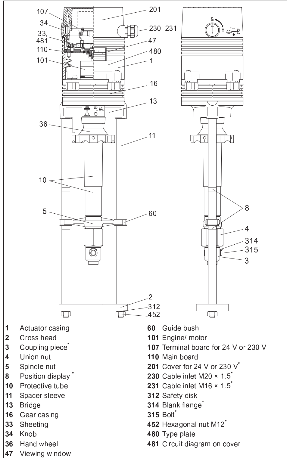
Diagram 1 Component drawings
