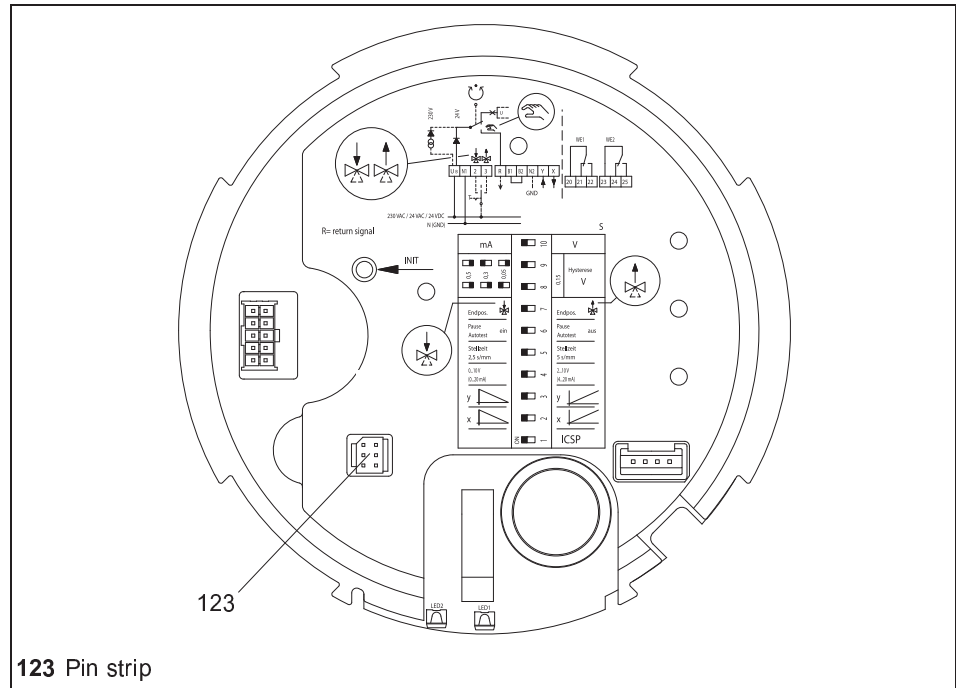
Diagram 12 Pin strip for way-switch printed circuit board on the motherboard
